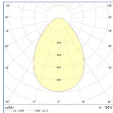
TERRA PANTRiA 3700 Flat
